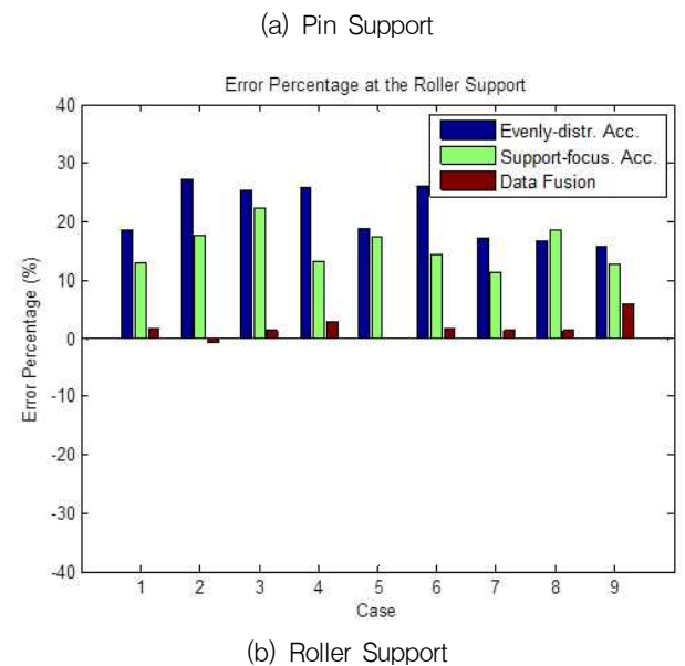
Fig. 6 Error Percentage of Updated Rotational Stiffness of Supports
