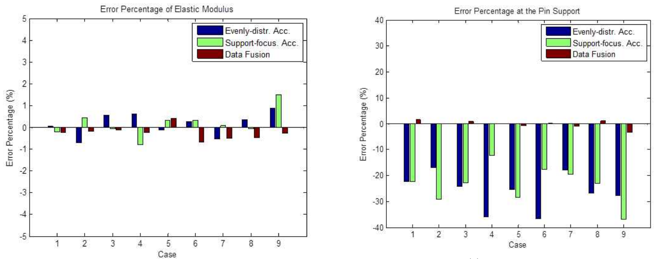
Fig. 5 Error Percentage of Updated Elastic Modulus
