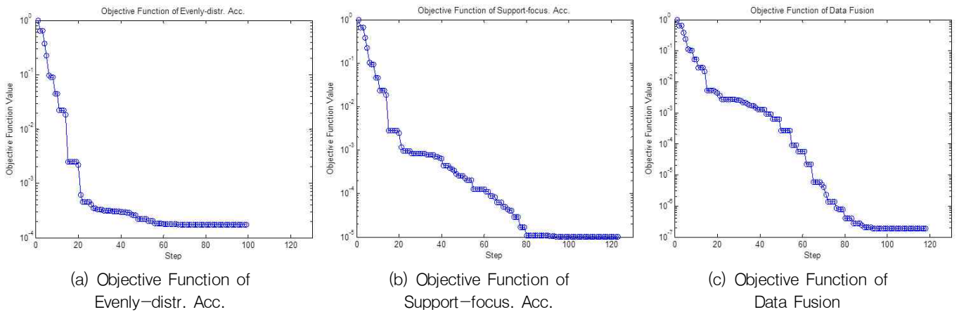
Fig. 4 Conversions of Objective Functions for 3 Measurement Scenarios
